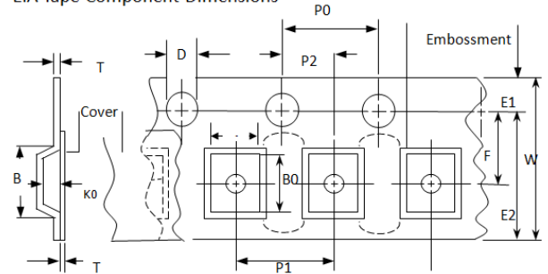
EIA Tape Component Dimensions
