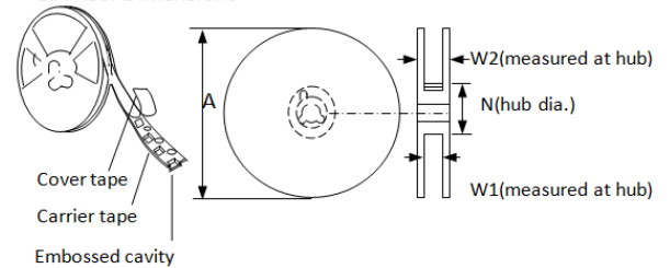
EIA Reel Dimensions
